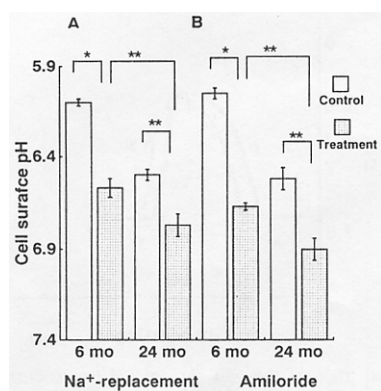
Fig. 3. Effects of Na + -replacement and 1 mM amiloride on the cell surface pH of the proximal jejunum in the young-adult and the senescent rats. After 5 min perfusion with the standard solution, when the control measurements were carried out, the perfusion solution was changed to the Na + -free solution (A) or a solution 1 mM amiloride containing (B), and the cell surface pH was recorded after 15 min. Results are presented as the mean ± S.E. of 10 separate experiments. Statistical significance: * P < 0.01 , ** P < 0.05 .
